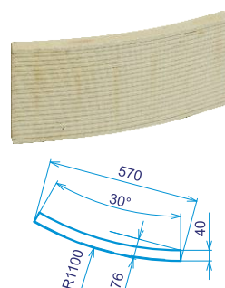
AK-OA1100 - Oblouk R1100 10,3kg
