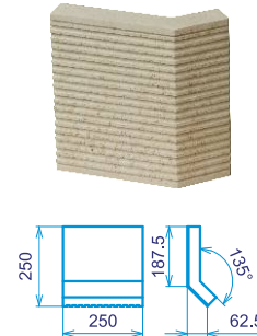
AK-ZA010 - Roh 135° 500x500x40 - 4,94kg
