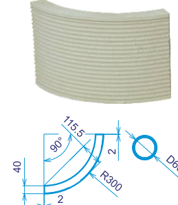
AK-OA300 - Oblouk R300 8,25kg
