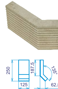
AK-ZA011 - Roh 135 500x125x40 - 2,48kg
