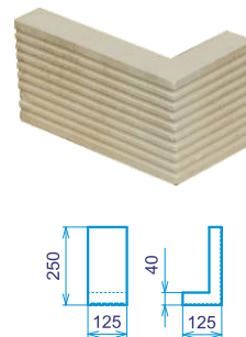
AK-RA011 - Roh 90 125x125x125 - 3,12kg
