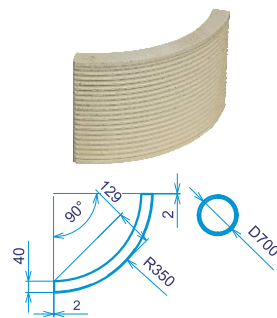
AK-OA350 - Oblouk R350 9,71kg
