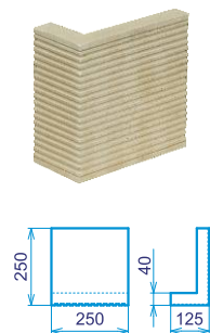
AK-RA010 - Roh 90 250x250x125 - 6,24kg
