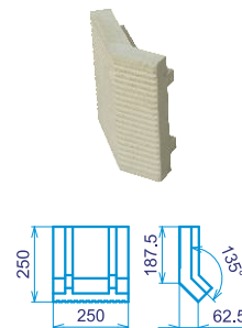
AK-ZV010 - Roh 135 250x250x125x40 - 7,52kg
