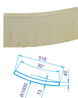
AK-OA1000 - Oblouk R1000 9,7kg
